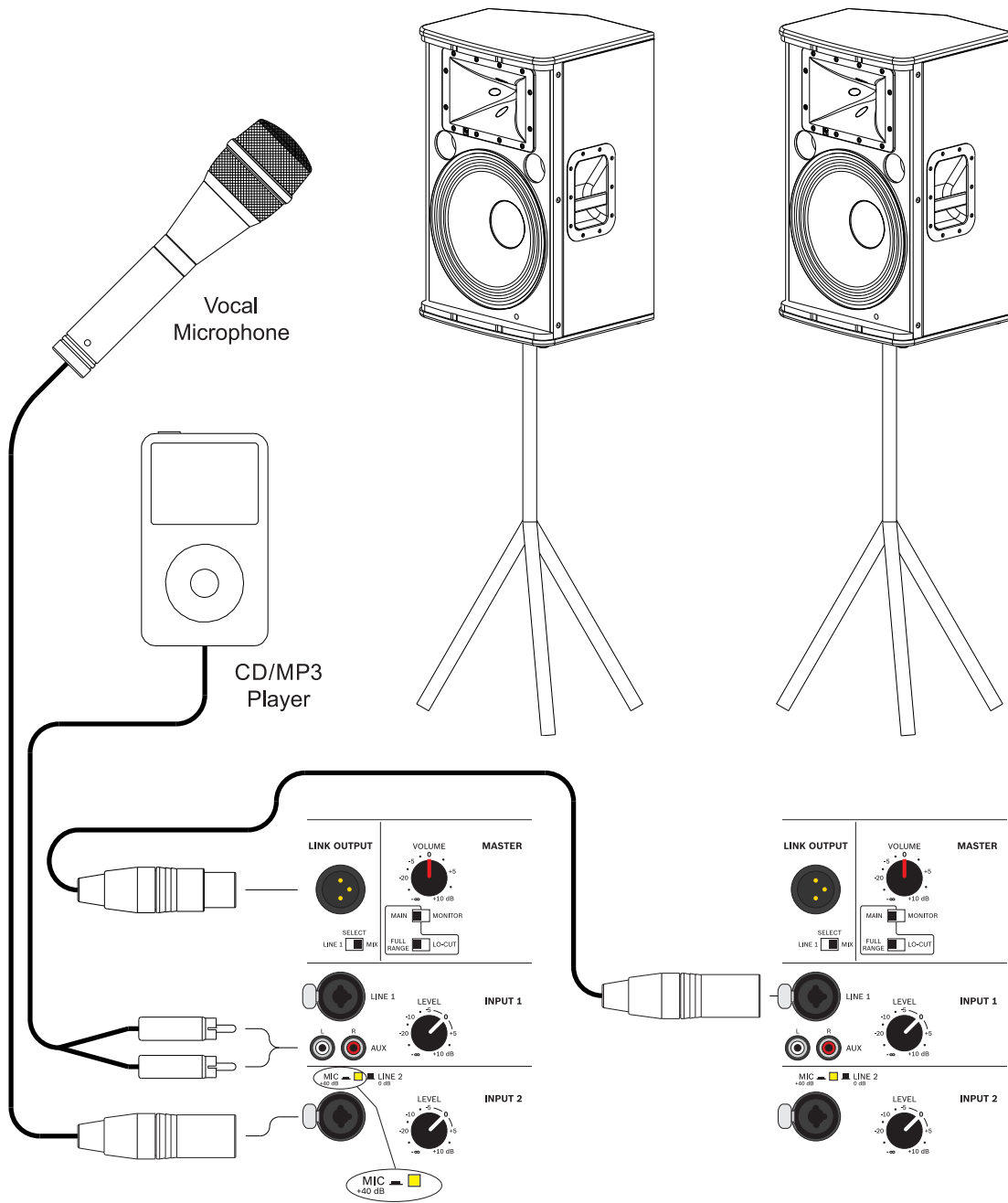
Illustration 3-7: Daisy-chaining full-range systems (dual A 112A or A 115A)
