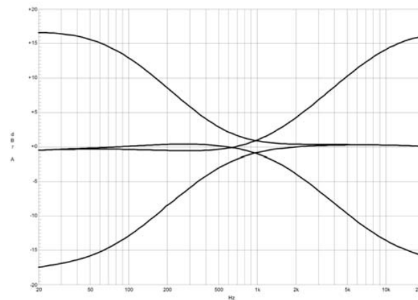
Illustration 2-7: LO/HI filters
