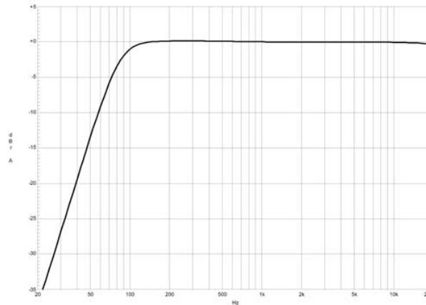
Illustration 2-5: LO CUT filter
