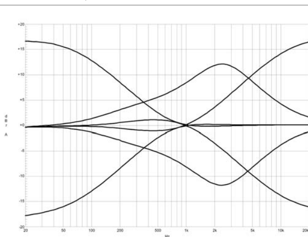
Illustration 2-16: HI, MID and LO filters
