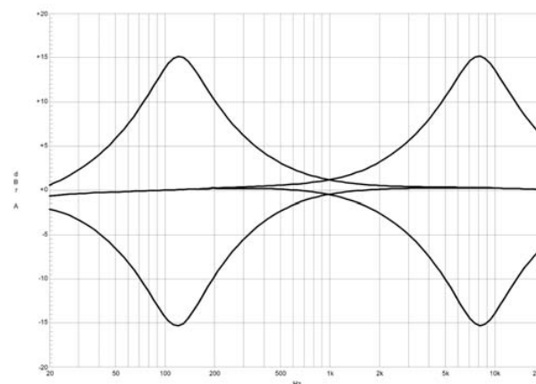
Illustration 2-8: MID filter
