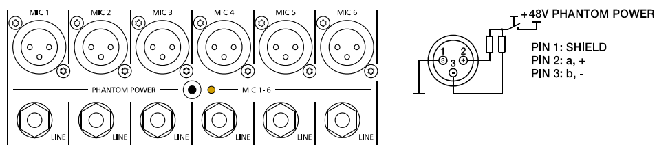
Illustration 2-1: Microphon input
