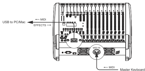
Illustration 4-10: Using the PC/Mac as MIDI tone generator
