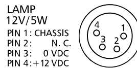
Illustration 2-18: Pin assignment of LAMP 12V/5W output
