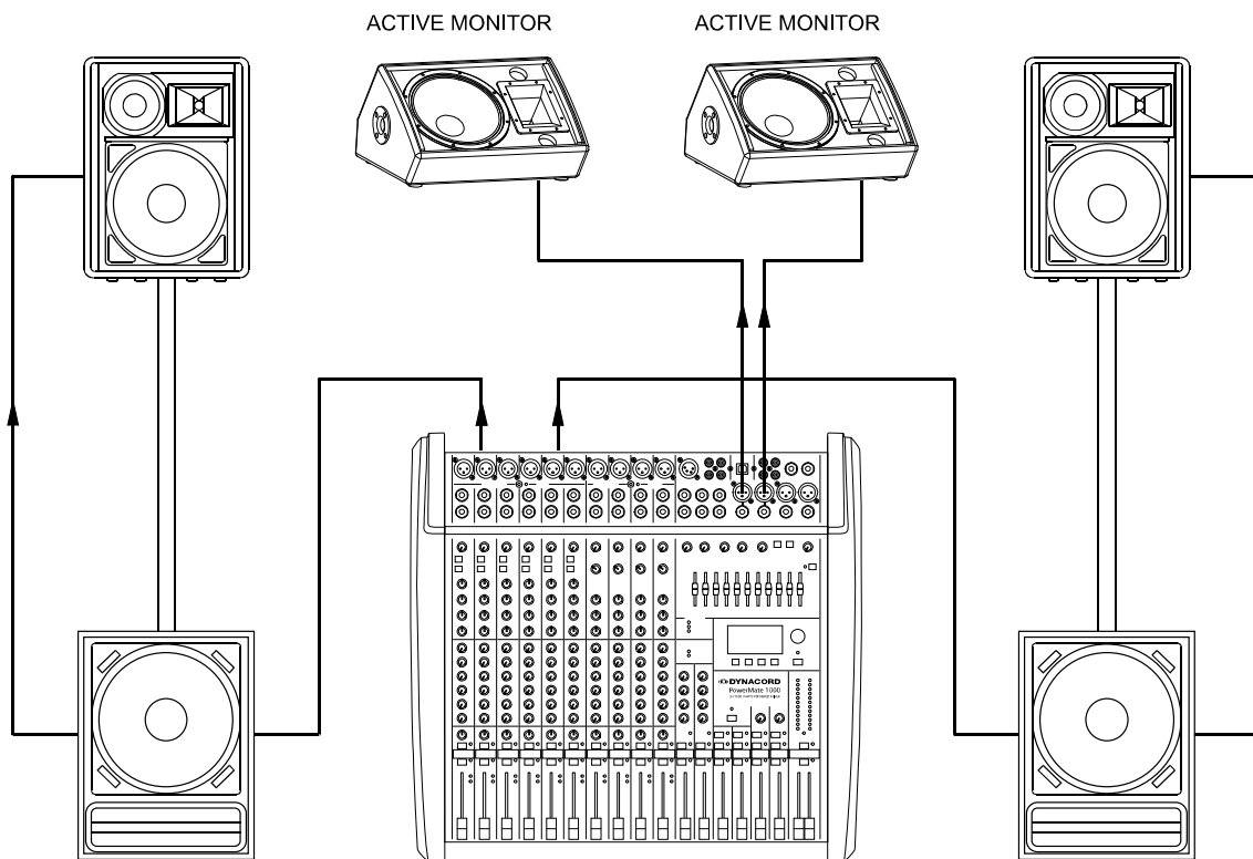
Illustration 5-1: Setting up a standard PA-system
