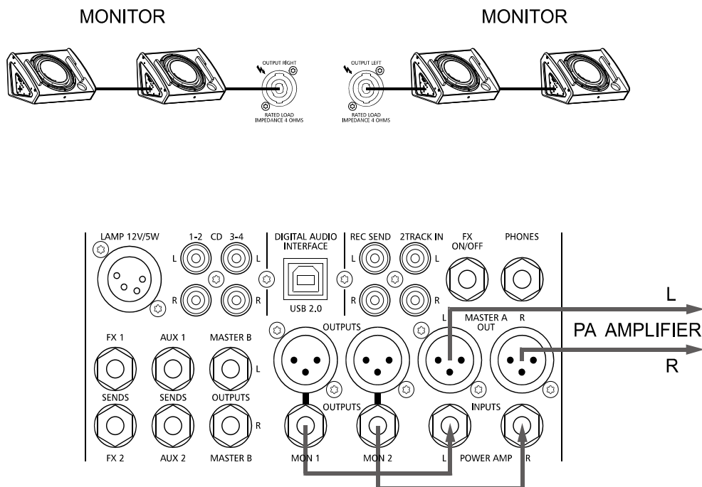
Illustration 6-3: Using internal power amplifier for monitoring purposes
