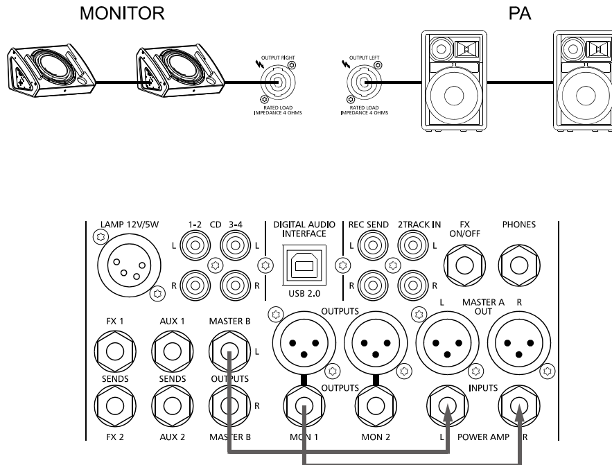
Illustration 6-4: Mono PA + Monitor
