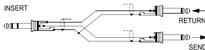
Illustration 2-3: Y cable for Insert jack
