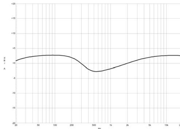
Illustration 2-6: Voice filter
