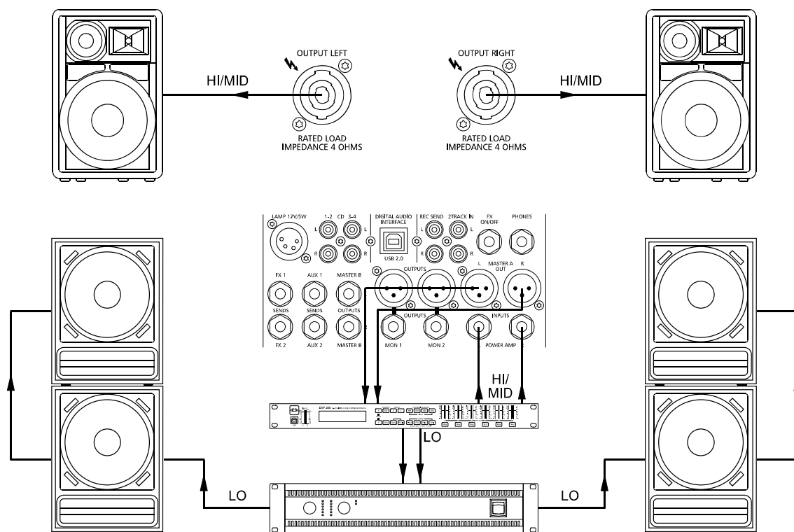
Illustration 6-5: Active 2-way stereo configuration
