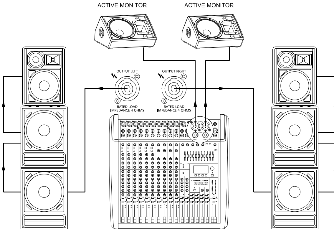
Illustration 6-1: Maximum amount of speakers in passive configuration
