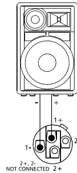
Illustration 2-20: Connection of a passive speaker
