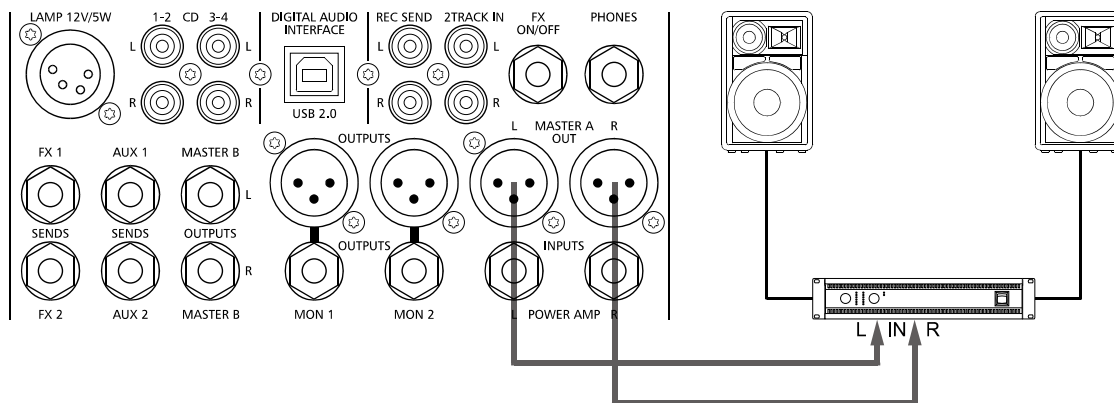
Illustration 6-2: Connection of an external power amplifier at MASTER A OUT L/R
