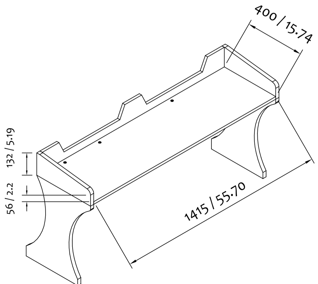
KEYBOARD TRAY
