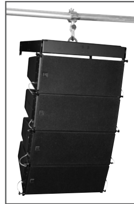
Fig. 17: Hoisting the top four CAD 208 enclosures
