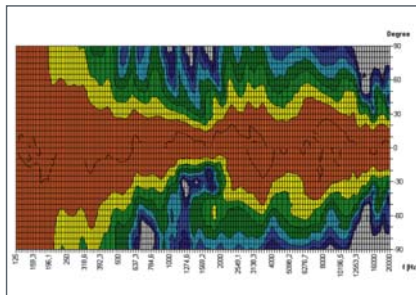
CAD 208 Directivity vertical 2D
