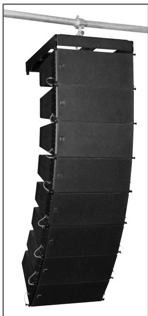
Fig. 18c: Mounting additional CAD 208 cabs: Mounting block b
