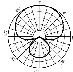
SUPERCARDIOIDE
