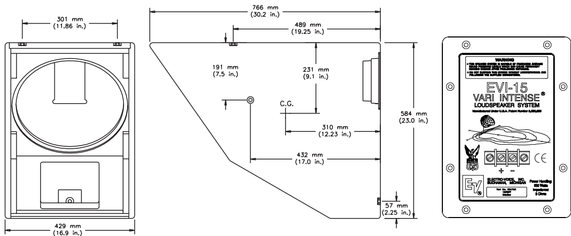
Figure 9—EVI-15 Dimensions
