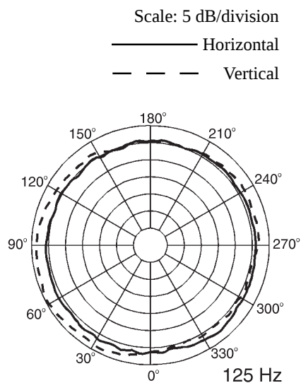
Figure 5—EVI-15 Polar Response
