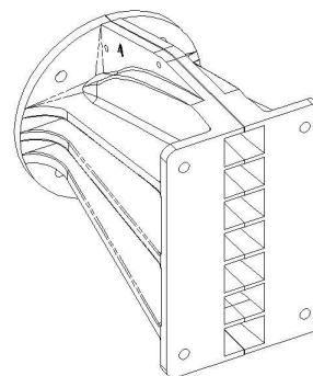
Figure 3-7 Hydra™ plane-wave generator
